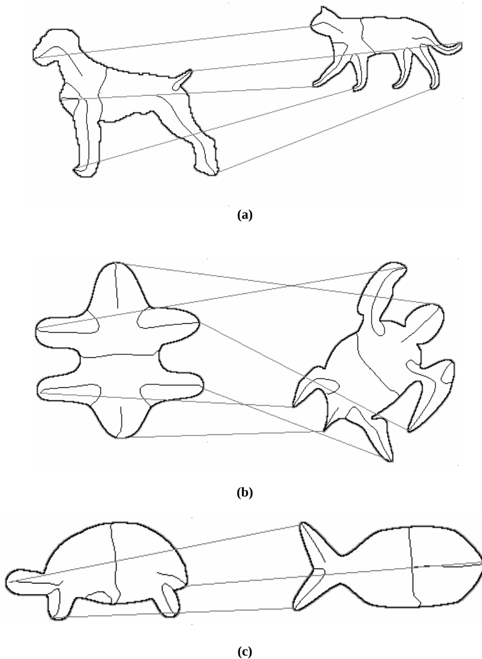
Figure 6-8 Correspondences between shape pairs belonging to different categories. The similarity scores detected are (a) 0.28 (b) 0.81 (c) 0.32.
